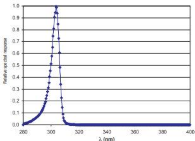
Typical spectral response curve LP UVB 03BLAV
