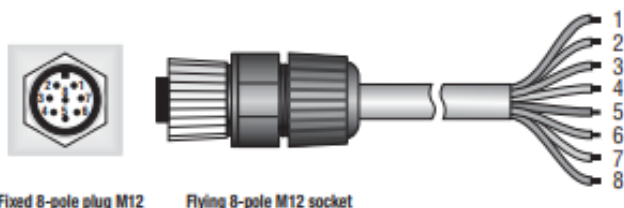
Fixed 8-pole plug M12
