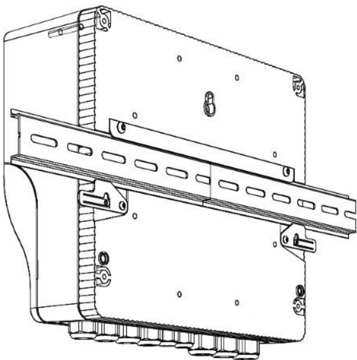
Fig. 4 Rail-DIN mounting
