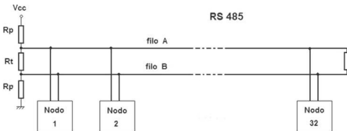
Termination with pull-up and pull-down resistances.
