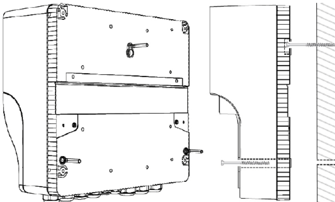
Fig. 2 Wall mounting
