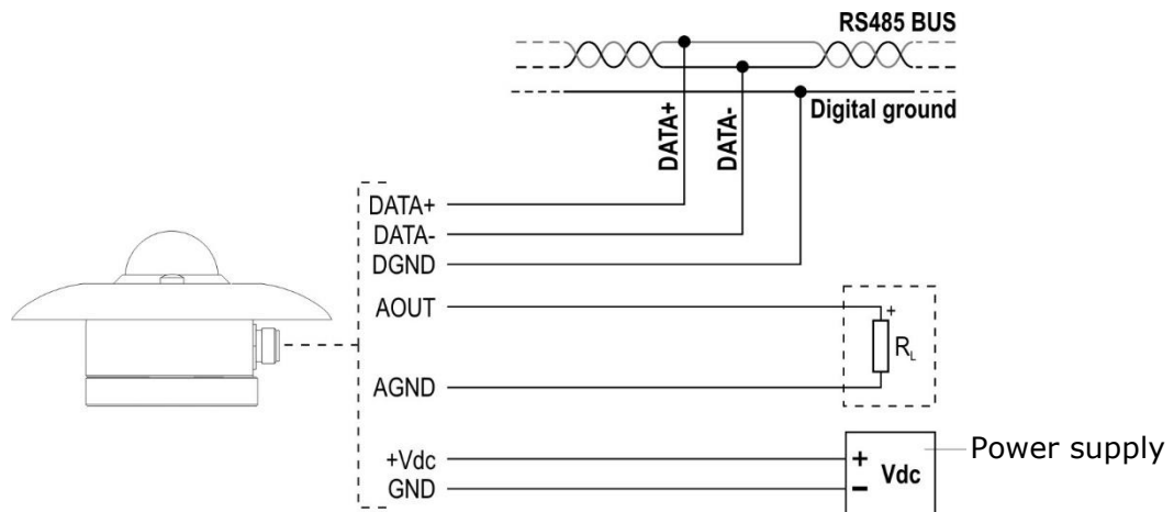
Fig. 4.4: LPS03Mxx connection diagram
