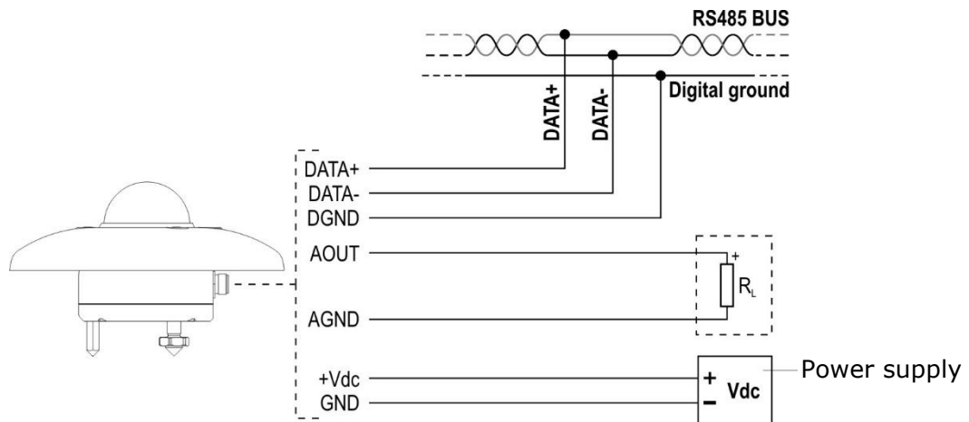
Fig. 4.4: LPS10Mxx connection diagram
